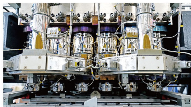
6-Fold ReCo 3-layer Extrusion Head, with View Stripe
